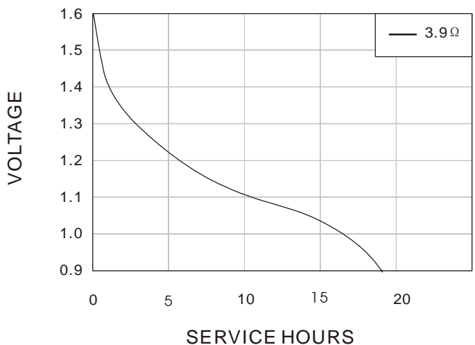
TYPICAL DISCHARGE CHARACTERISTICS AT 21^\circ\text{C} ( 60 \pm 15\%\text{RH} )
